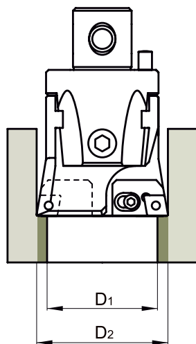
Symmetrical boring
